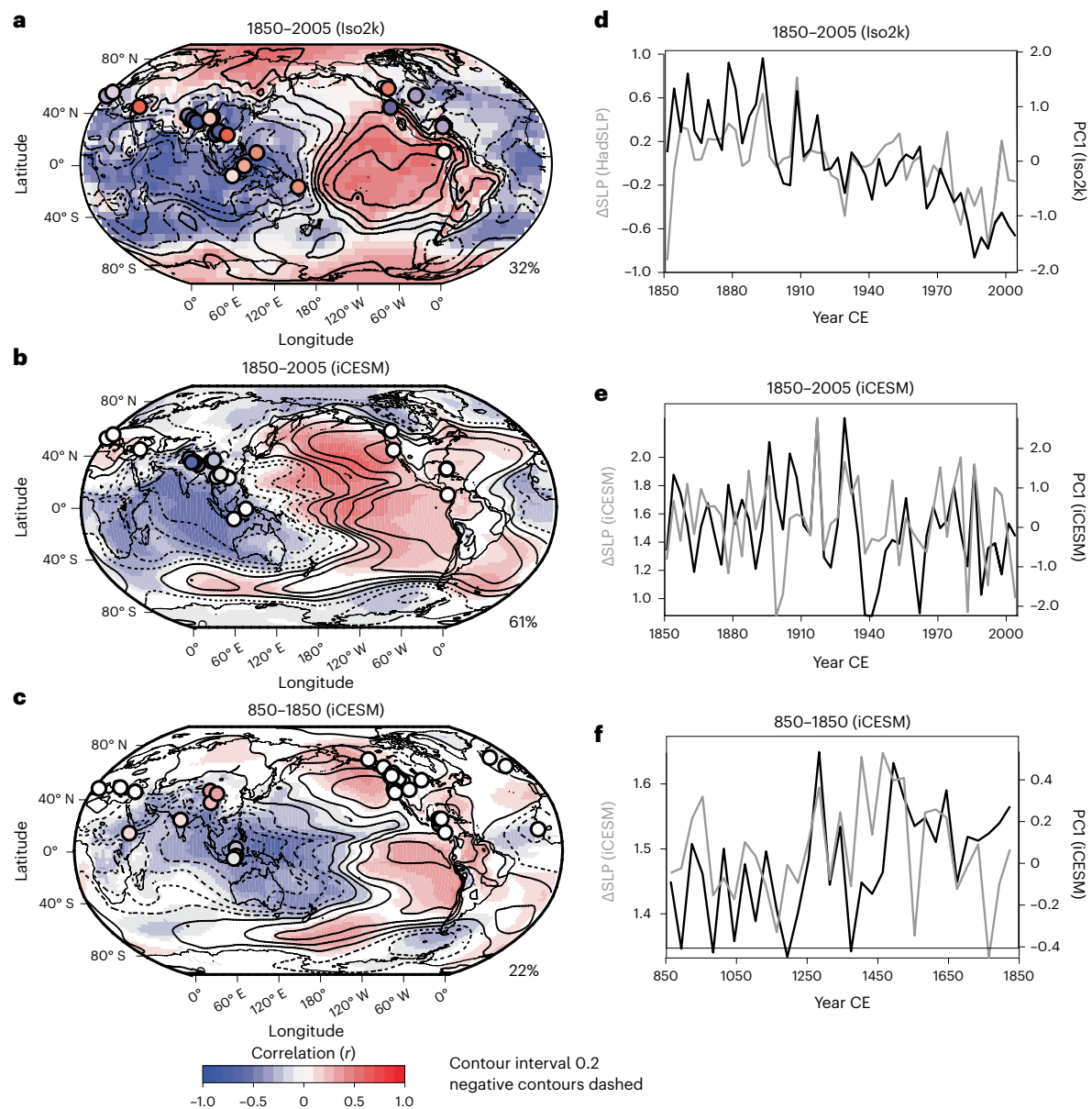
Fig. 4 | Isotopic fingerprint of the PWC in Iso2k and iCESM. a , Shading is the correlation between observed SLP and PC1 of three-year binned Iso2k EM records (1850 to 2005). Symbol colours denote site loading on PC1. Unfilled contours denote correlation between SLP and PWC index ΔSLP. b , Correlation between SLP and ensemble mean PC1 of three-year binned 0–10 cm \delta^{18}\text{O}_{\text{soil}} in iCESM
