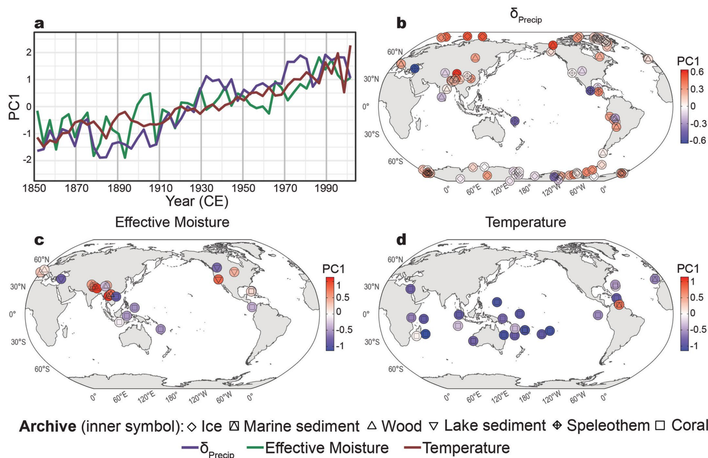
Extended Data Fig. 8 | First Principal Component (PC1) of Iso2k 15 data for the Historical Period. Panels a–d, as in Extended Data Fig. 3a–d, but for the interval 1850–2005, with 3-year bins. \delta_{\text{precip}} PC1 explains 12% of the total variance (n = 109).
