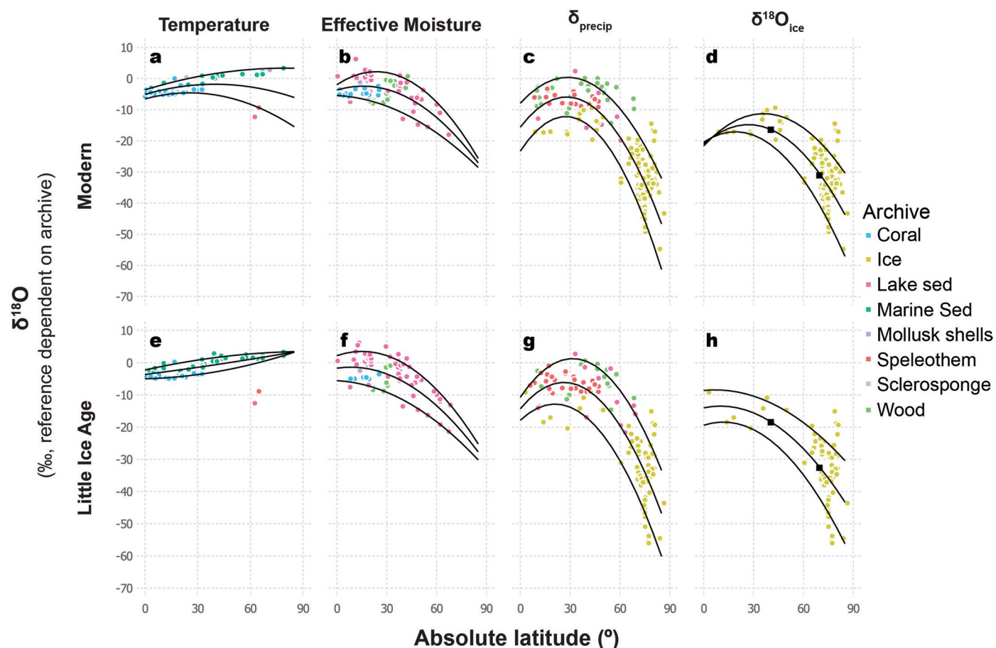
Extended Data Fig. 5 | \delta^{18}\text{O} vs. latitude in the Iso2k database 15 for the modern era (a–d; 1950–2018) and the Little Ice Age (e–h; 1450–1850). Data are plotted for the three main isotope interpretation categories (a–c, e–g) and for \delta^{18}\text{O} of glacier and ground ice (d, h), the archives that preserve precipitation most directly. Black lines indicate polynomial fits to the 0.1, 0.5, and 0.9 quantiles. Black
