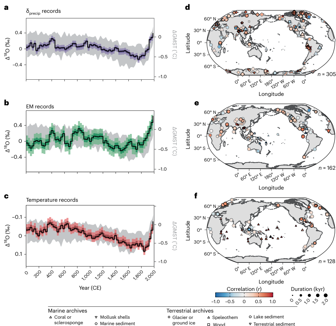
Fig. 1 | Global composite oxygen isotope anomalies. a–c , 30-year binned proxy \Delta^{18}\text{O} (black line, ensemble median; dark shading, 25th–75th percentiles; light shading, 2.5th–97.5th percentiles) for each group of Iso2k records 15 , anomalies relative to 2,000-year mean. Grey shading depicts ensemble 2.5th–97.5th percentile GMST anomaly relative to 1961–1990 mean 1 . Note y axis in c is reversed
