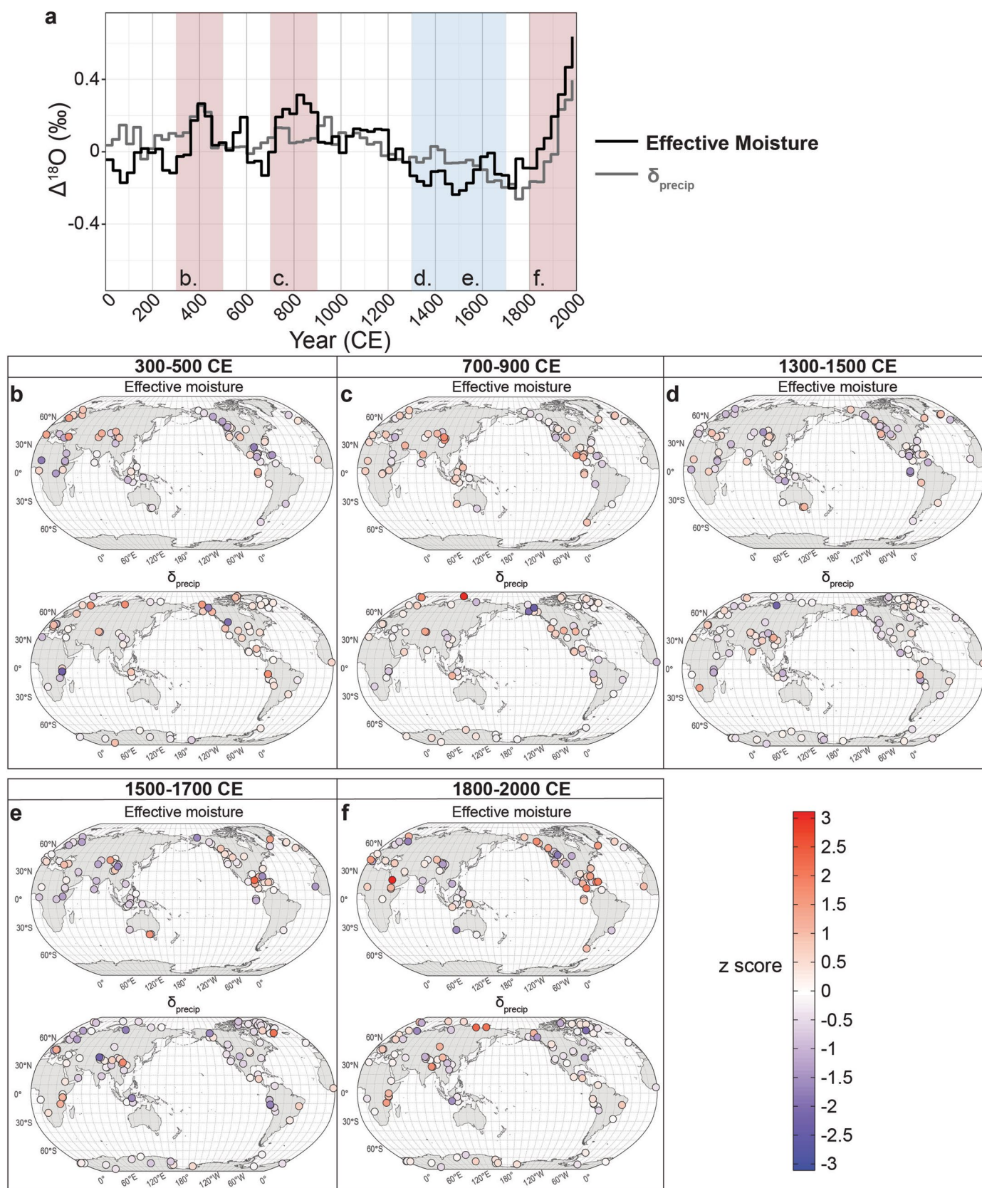
Extended Data Fig. 7 | Standardized 200-year \delta^{18}\text{O} anomalies from Effective Moisture and \delta_{\text{precip}} records. a , Composite medians for Iso2k 15 Effective Moisture and \delta_{\text{precip}} driven records, as shown in Fig. 1 of the main text. Red shading denotes intervals of relatively high composite \delta^{18}\text{O}_{\text{EM}} , and blue shading denotes intervals of relatively low composite \delta^{18}\text{O}_{\text{EM}} . b-f , Isotopic anomalies in individual
