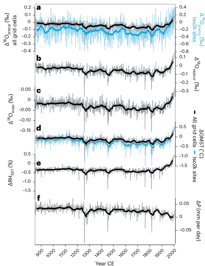
Fig. 3 | Global hydroclimate and isotopic anomalies in iCESM 18–20 . a , Ensemble mean, amount-weighted mean annual \Delta^{18}\text{O}_{\text{precip}} anomaly relative to 1961 to 1990 mean (thin grey line) and 30-year running mean (thick black line) for all grid cells and for only grid cells containing Iso2k site locations (blue lines). Note, right y axis in a is scaled 2\times that of the left. b–f , As in a , but for global column-averaged \Delta^{18}\text{O}_{\text{vapour}} ( b ), \Delta^{18}\text{O} of evaporative flux from the global oceans ( c ), GMST ( d ), relative humidity over the low- and mid-latitude oceans ( 60^{\circ}\text{N} – 60^{\circ}\text{S} ) with respect to saturation vapour pressure at sea surface temperature ( \text{RH}_{\text{SST}} ) 13,29,30 ( e ) and global precipitation rate ( P ) ( f ).
