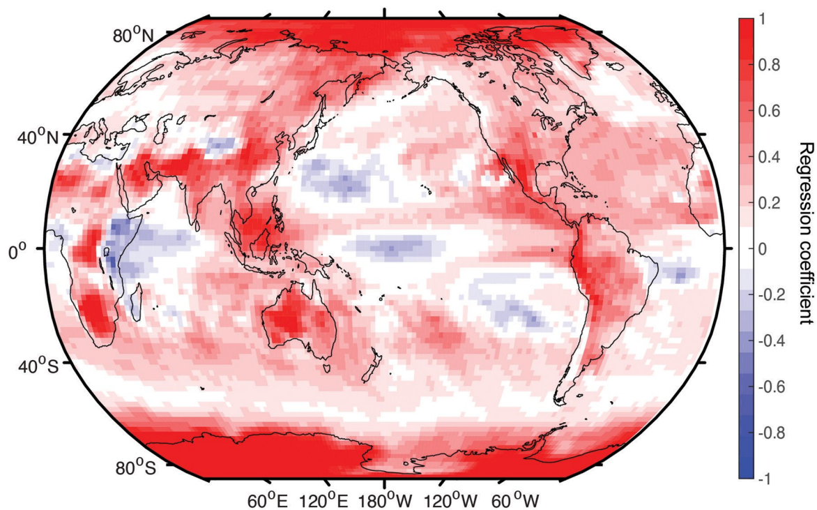
Extended Data Fig. 4 | iCESM relationship between GMST and grid cell-level \delta^{18}\text{O}_{\text{precip}} . Shading depicts the regression coefficient in \text{‰}/^{\circ}\text{C} between mean annual, amount-weighted, 30-year running mean \delta^{18}\text{O}_{\text{precip}} at every grid cell
