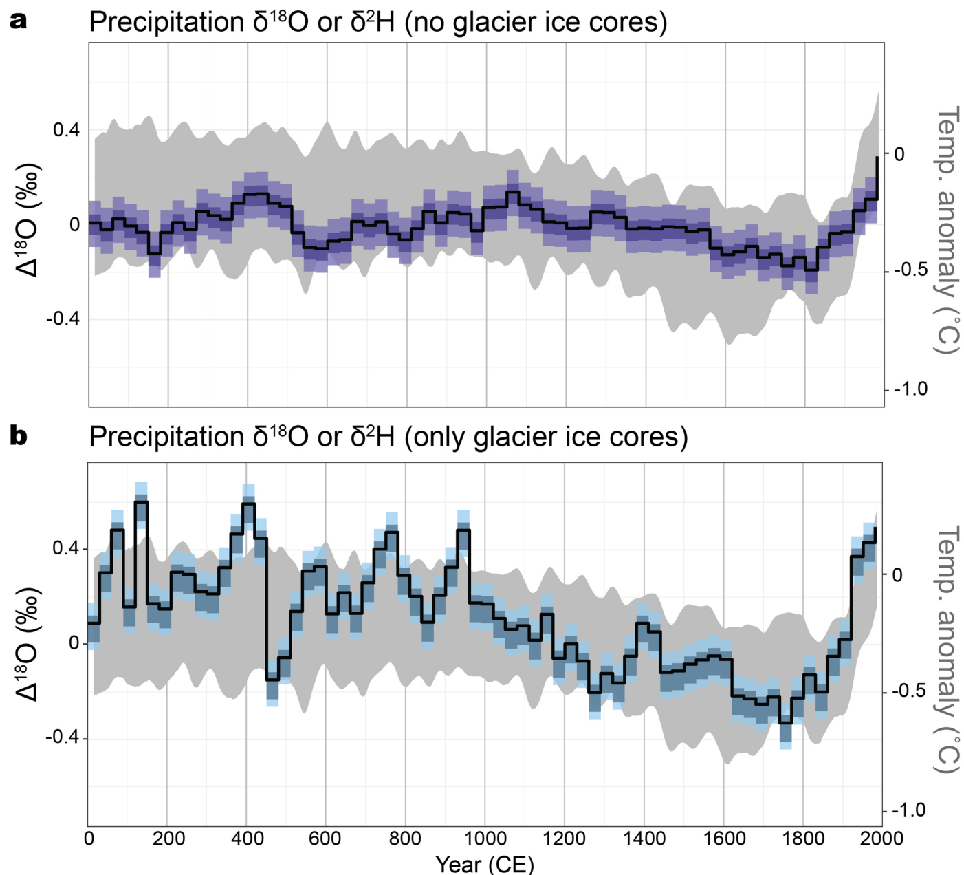
Extended Data Fig. 1 | Composite \Delta^{18}\text{O}_{\delta\text{precip}} calculated with and without glacier ice records. As per Fig. 1, the black line with coloured shading shows the 30-year binned proxy \delta^{18}\text{O} anomaly from Iso2k records 15 (black line, ensemble median; dark shading, first and third quantiles; light shading, 2.5th/97.5th percentiles). (a) Composite of \Delta^{18}\text{O}_{\delta\text{precip}} records from all archives other than glacier ice. (b) Composite of only glacier ice records. Records contributing to
