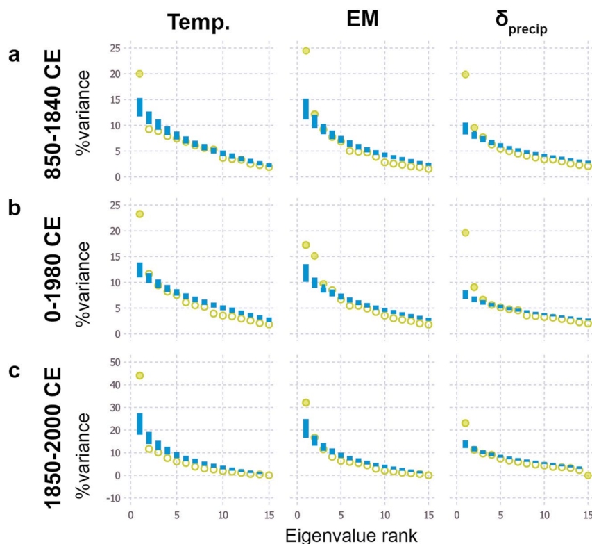
Extended Data Fig. 9 | Significance of Iso2k 15 PCA eigenvalues with respect to a null hypothesis of stochastic forcing with decadal persistence. a , Block bootstrap results from 850-1840 with a 30-year bin width, 10-year block length, and tolerance of up to 15% missing data (that is, 85% coverage during the time interval; Methods). Yellow symbols depict the eigenvalues (expressed as a percentage of the total variance) of each principal component. Blue bars show
