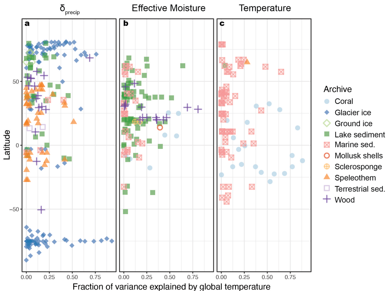
Extended Data Fig. 6 | Relation between Iso2k 15 primary time series and Global Mean Surface Temperature (GMST). (a) Fraction of variance explained ( R^2 ) in \delta_{\text{precip}} primary time series by changes in PAGES 2k global mean surface temperature (GMST) over the past 2000 years 12 . Both Iso2k time series and GMST
